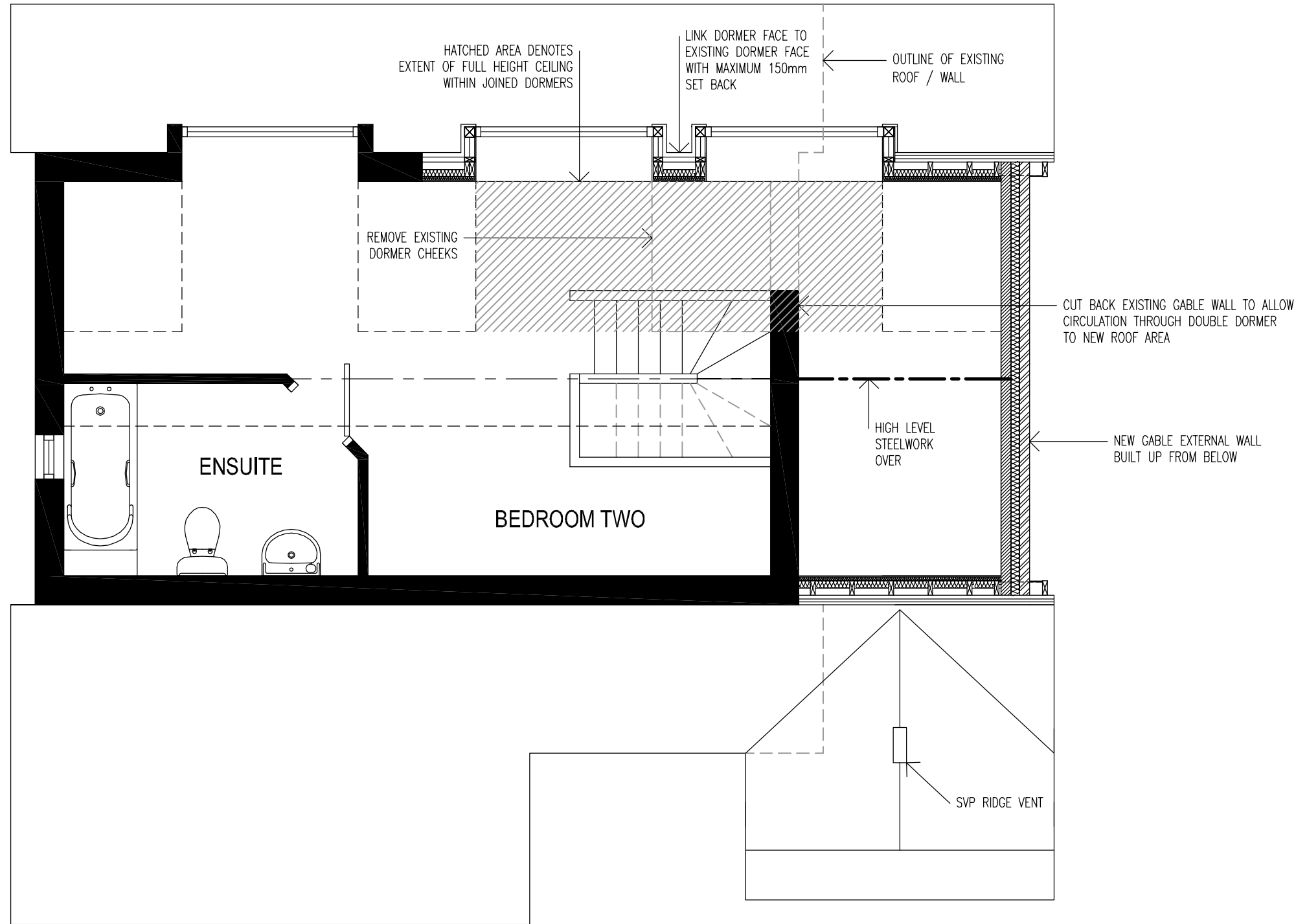
1:50 SECOND FLOOR PLAN
