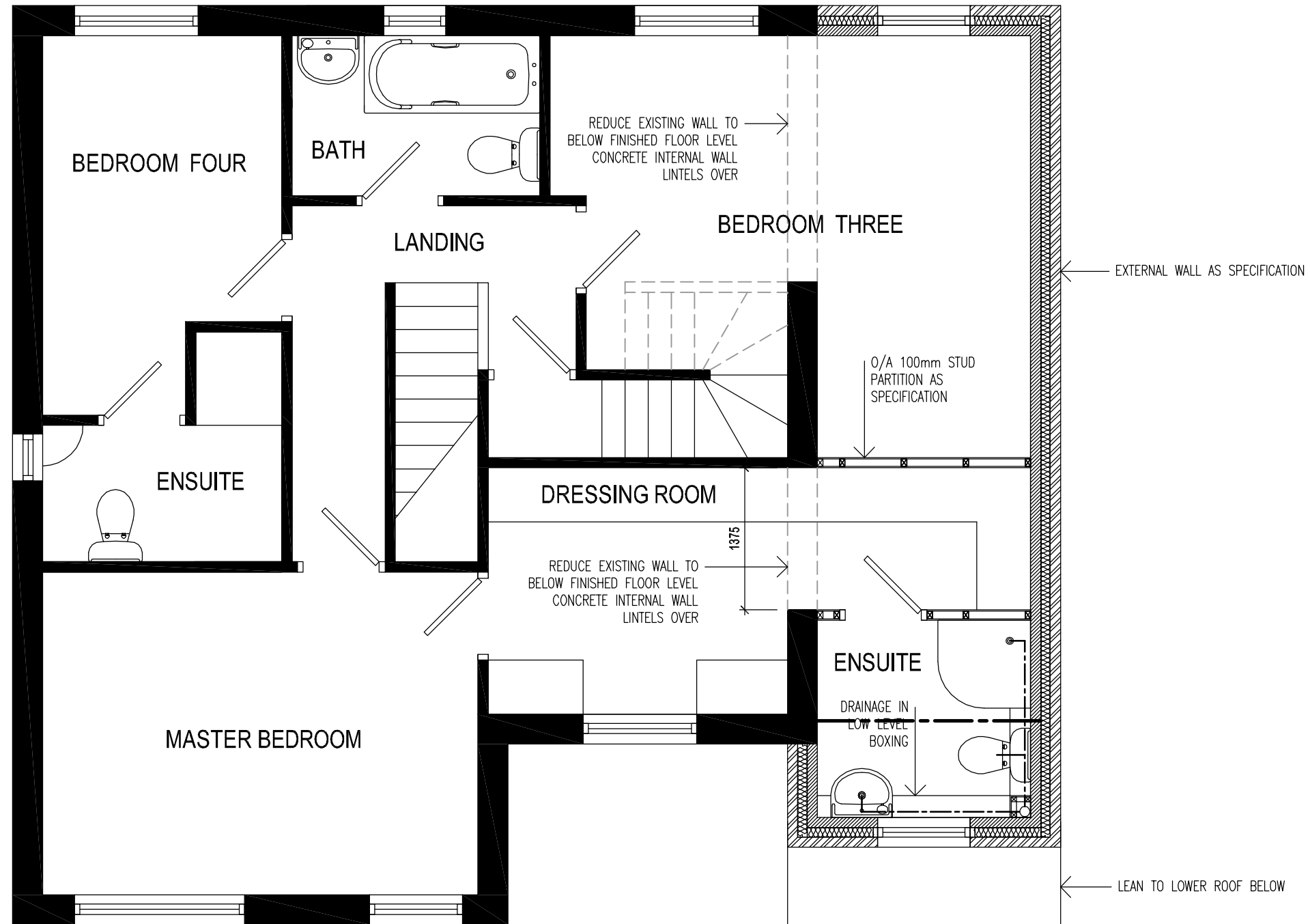
1:50 FIRST FLOOR PLAN
